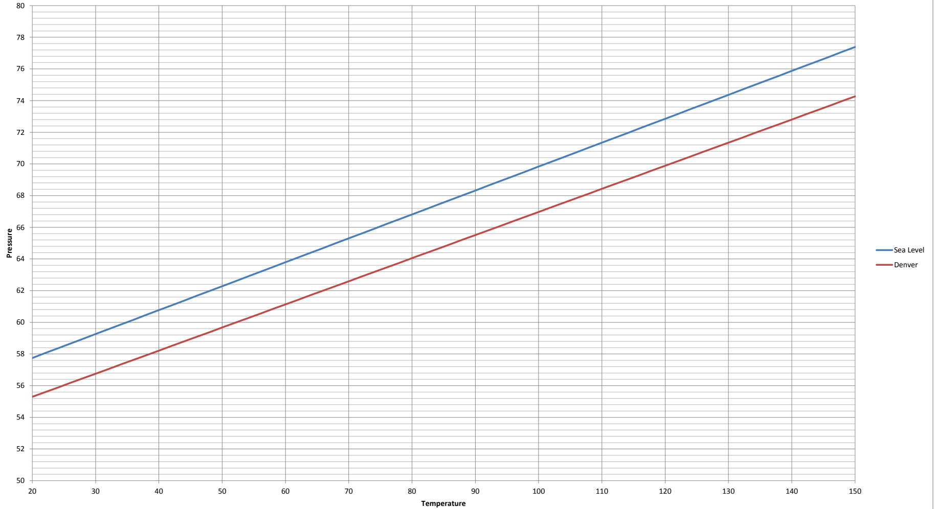
Pressure vs Temperature based on 65psi @ 68 degrees
